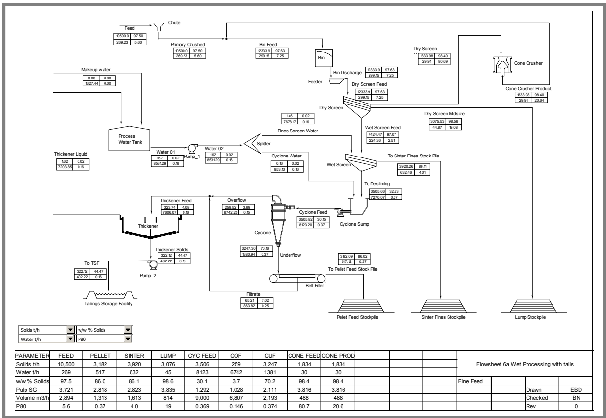
Typical Limn Flowsheet
