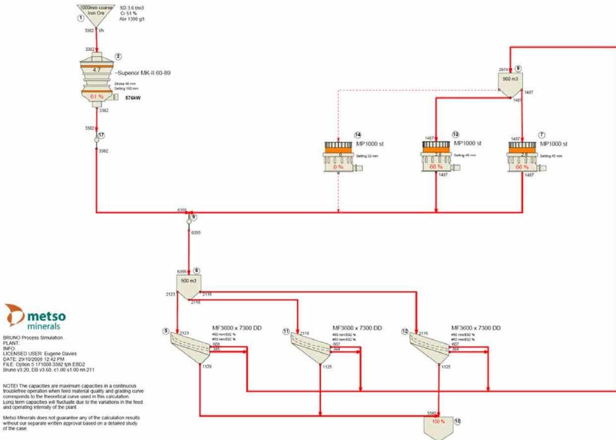
Typical Bruno Flowsheet
